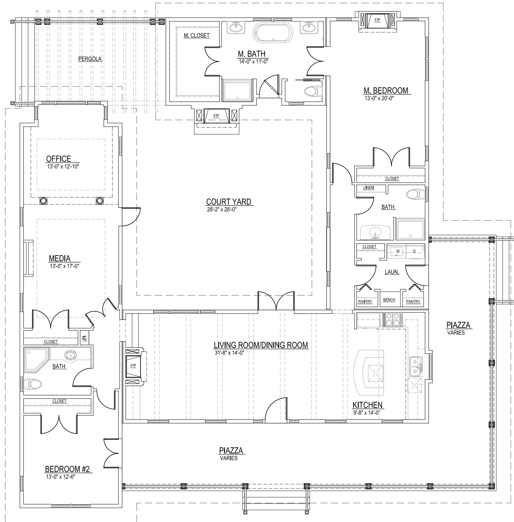
THE "WINDSOR" FIRST FLOOR PLAN
