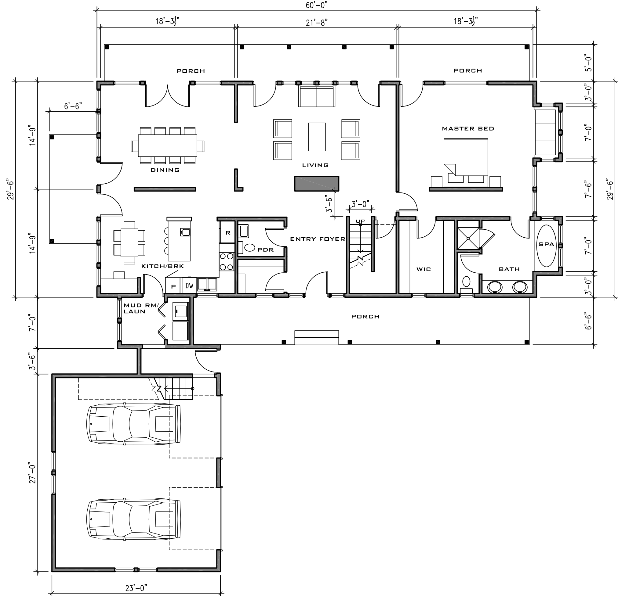
1 MAIN FLOOR PLAN 1/8" = 1'-0"
