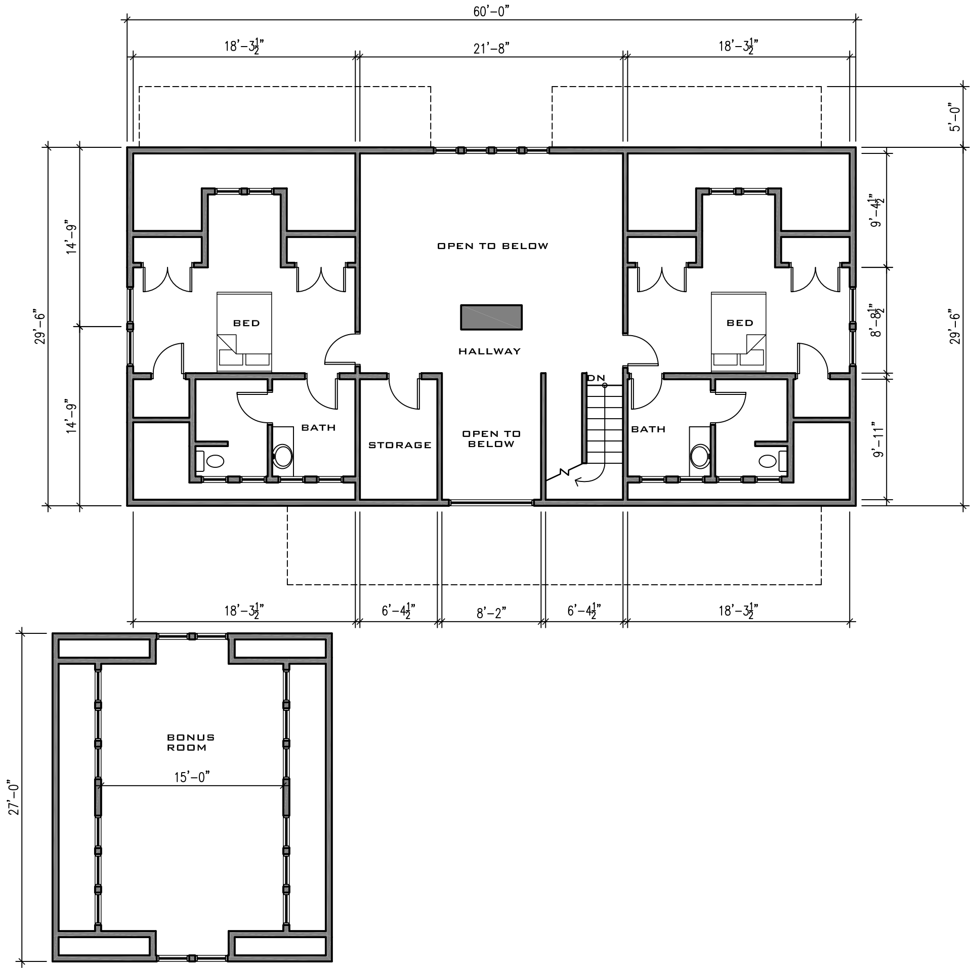
2 UPPER FLOOR PLAN 1/8" = 1'-0"
